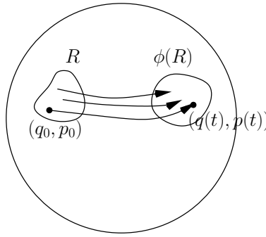
Figure 1.3: Hamiltonian flow.
