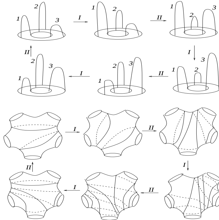
Figure 15: relation 9
