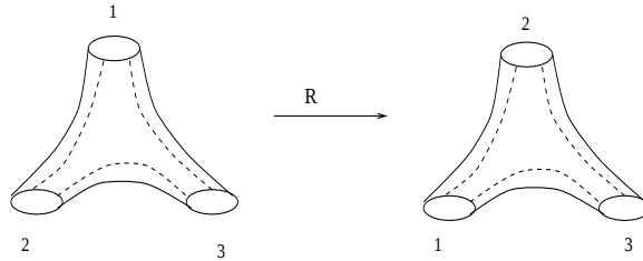
Figure 3: R
