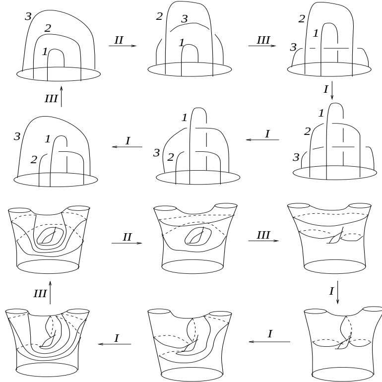
Figure 11: relation 2
