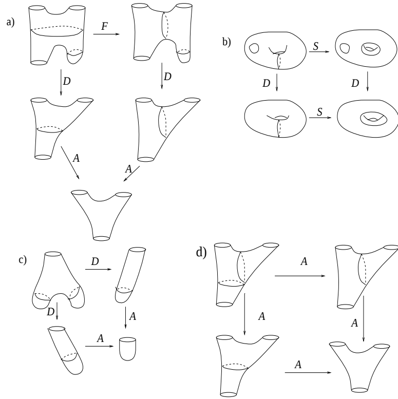
Figure 30: birth-death cells
