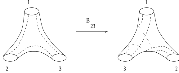
Figure 2: B_{23}
