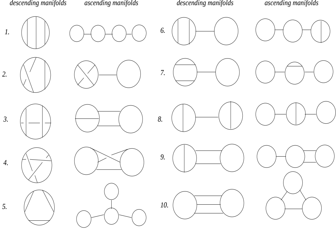
Figure 9: triangle singularities
